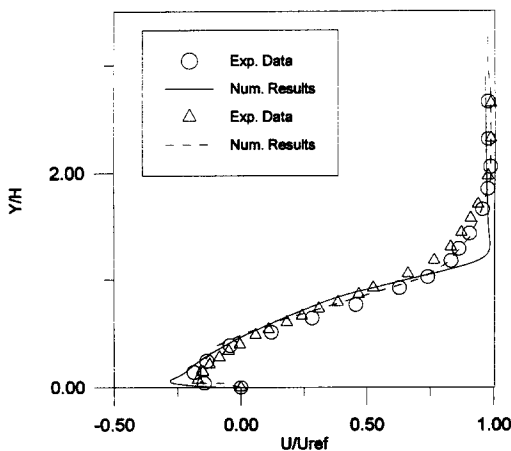
Fig. 7. Calculated velocity profiles for stations x^* = -0.32 ( \Delta , U_\infty = 10.33 \text{ m s}^{-1} ) and x^* = -0.44 ( \circ , U_\infty = 10.46 \text{ m s}^{-1} ). Data of Vogel and Eaton [10].
