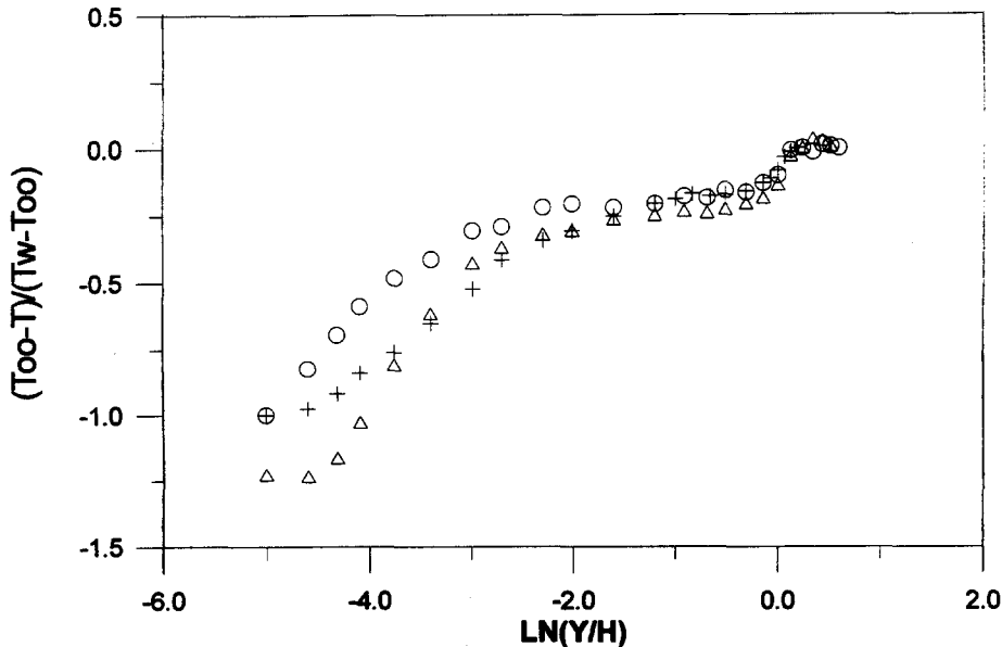
Fig. 3. Temperature profiles in reverse flow region according to Vogel and Eaton [10]. y is referred to the step height, H ( = 3.79 cm). The points were taken at stations x^* = -0.35 (○), -0.55 (△) and -0.75 (+), where x^* = (x - x_R)/x_R , x_R = 6.6643 H .
